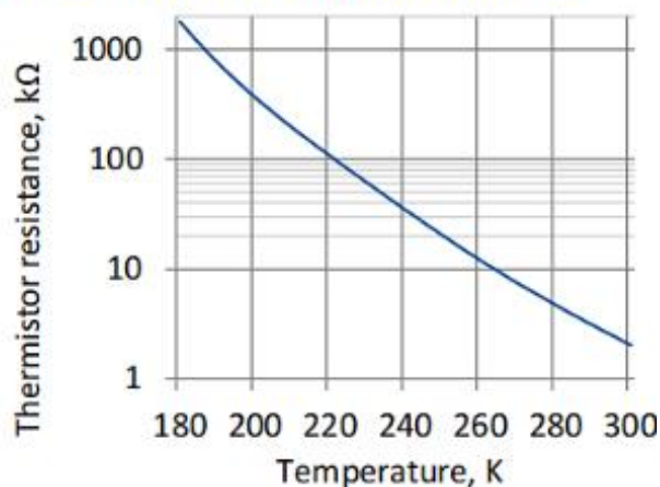
Thermistor characteristics
