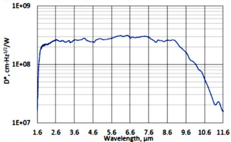
Spectral response ( T_a = 20^\circ\text{C} )
