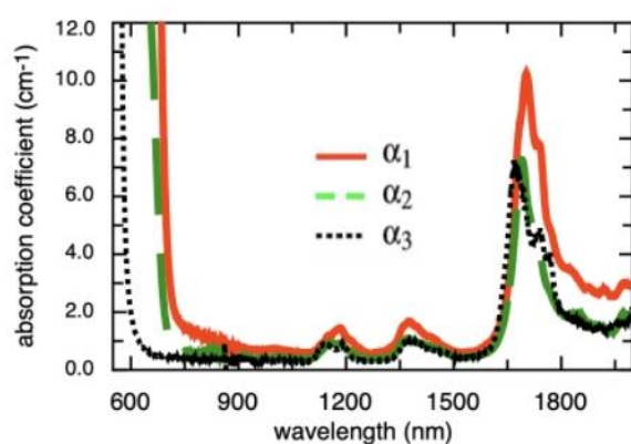
Absorption Spectrum
