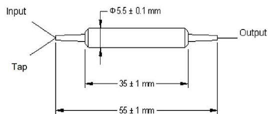
TypeB: Optical power for reflect band > 300 mW
