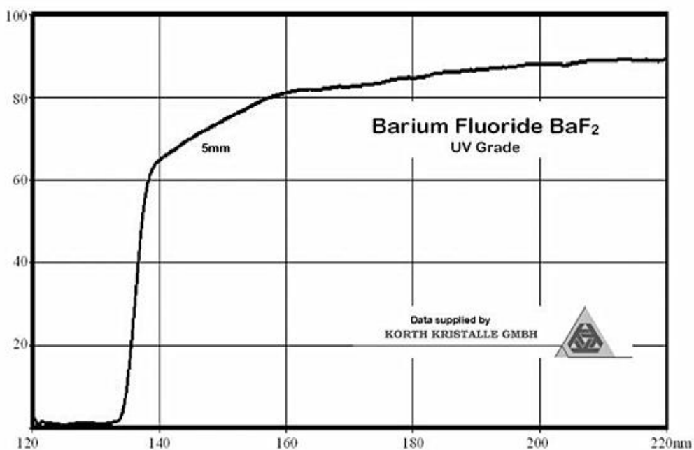
Transmittance \tau ( \lambda ) vs. Wavelength \lambda
